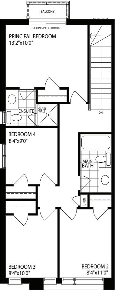
Third Floor Opt. 4 Bedroom Elevation A
