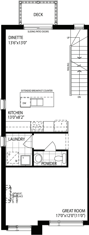
Second Floor Elevation B
