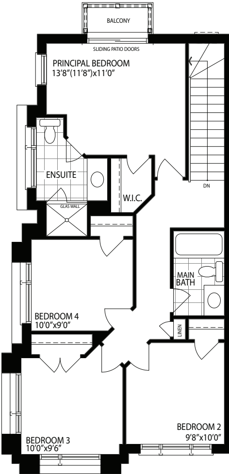
Third Floor Opt. 4 Bedroom Elevation A
