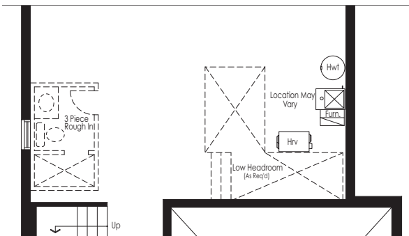
Optional Basement For Optional First Floor
