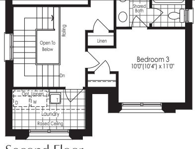
Second Floor Elevation C
