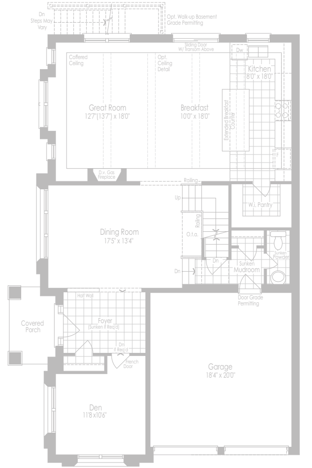
First Floor - Elevation C
