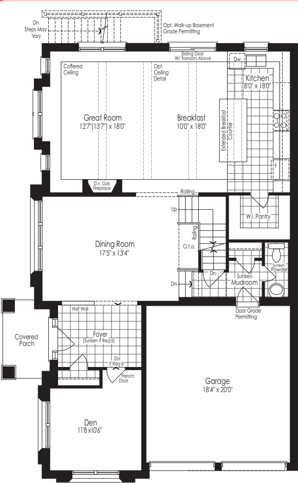
First Floor - Elevation C
