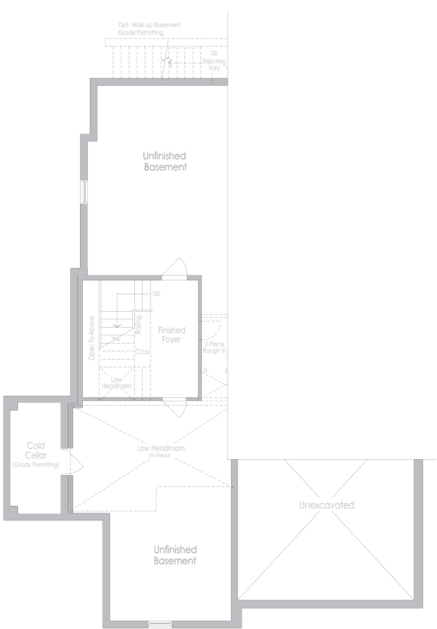
Basement Elevation C
