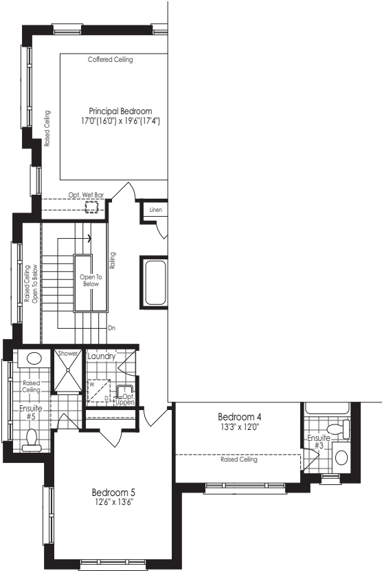
Opt. 5 Bedroom Second Floor Elevation B
