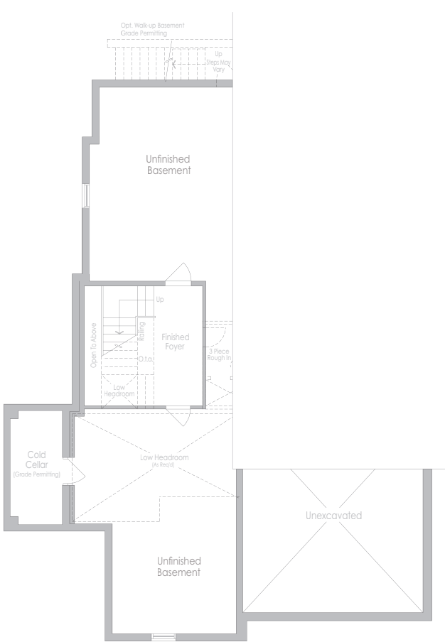
Basement Elevation C
