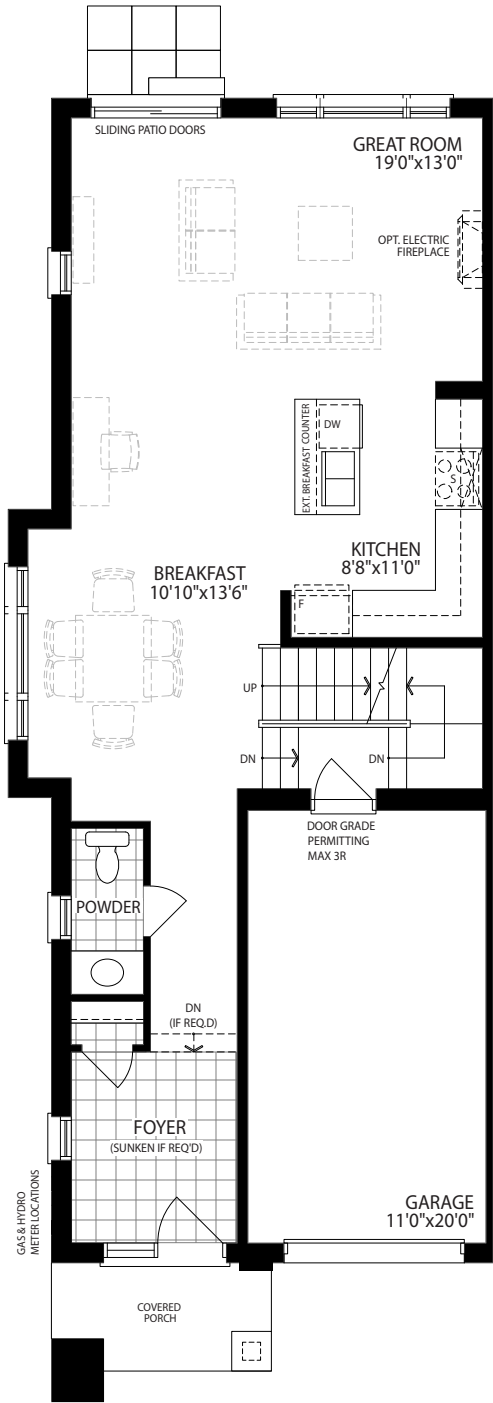
Ground Floor Elevation C1
