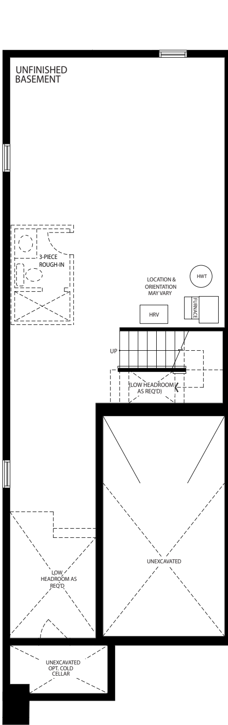
Basement Elevation C1
