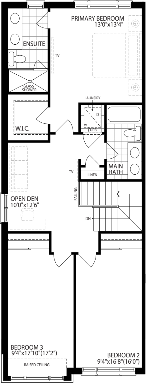
Second Floor Elevation C2
