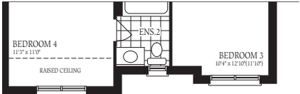
Second Floor - Elevation C
