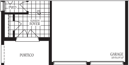
Ground Floor - Elevation C
