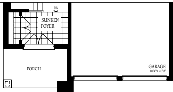
Ground Floor Elevation C
