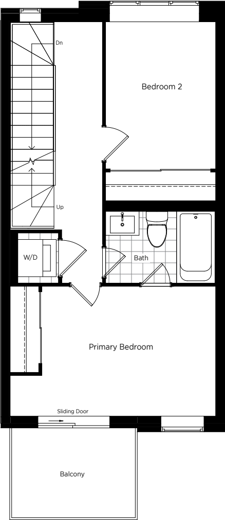
Third Floor
