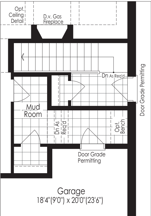
Optional Ground Floor Plan W/ Service Stairs 3,675 sq.ft. Elev. A 3,770 sq.ft. Elev. B & C
