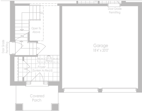
First Floor Elevation C
