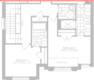
Opt. 5 Bedroom Second Floor Elevation C
