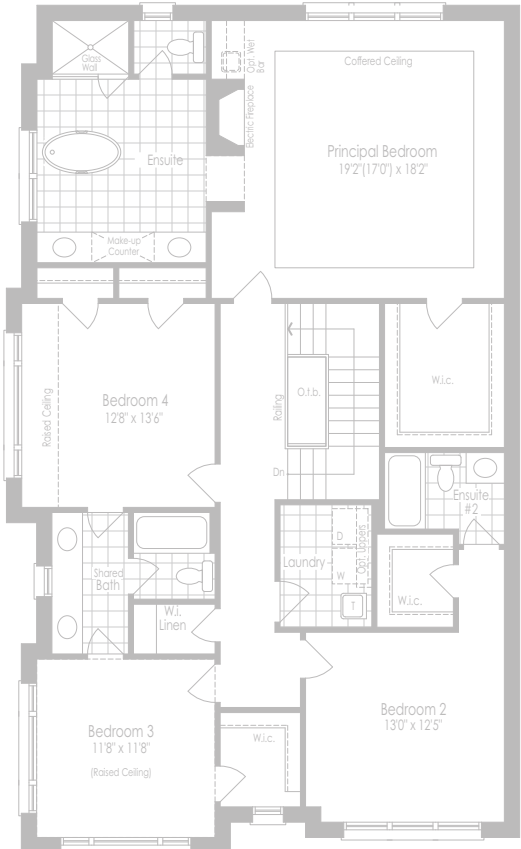
Second Floor - Elevation B
