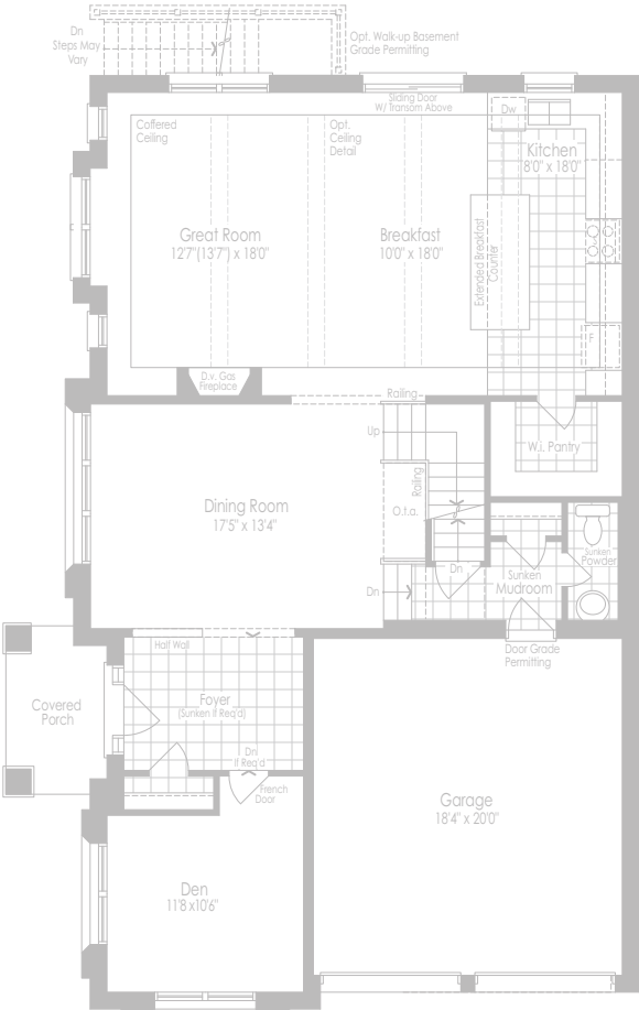
First Floor - Elevation C
