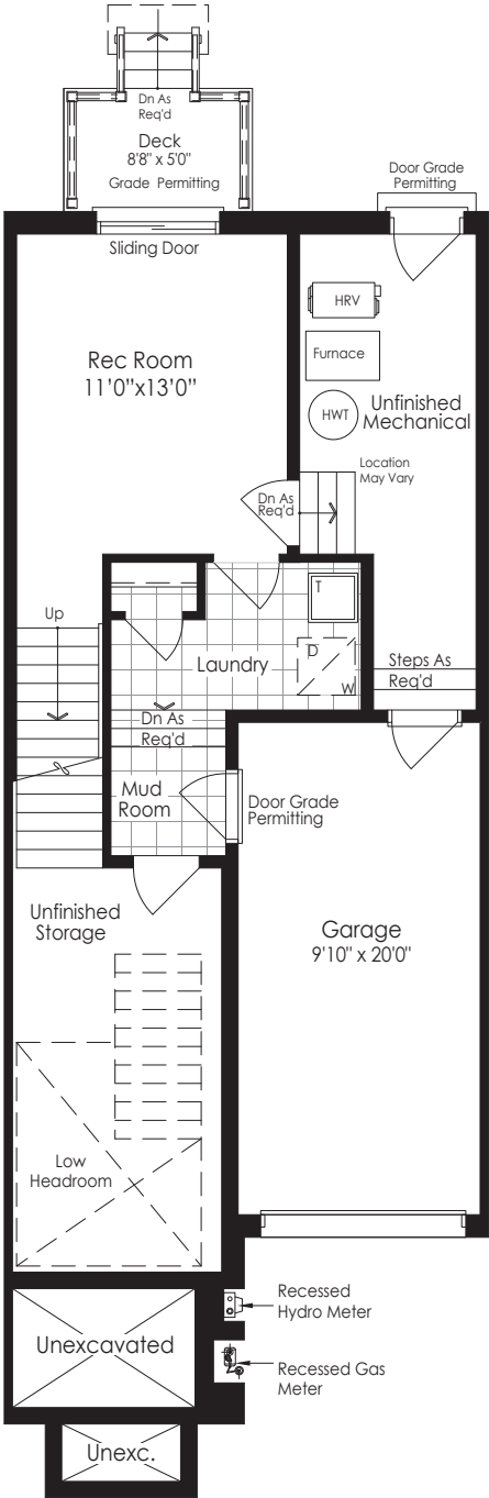
GROUND FLOOR Elevation A
