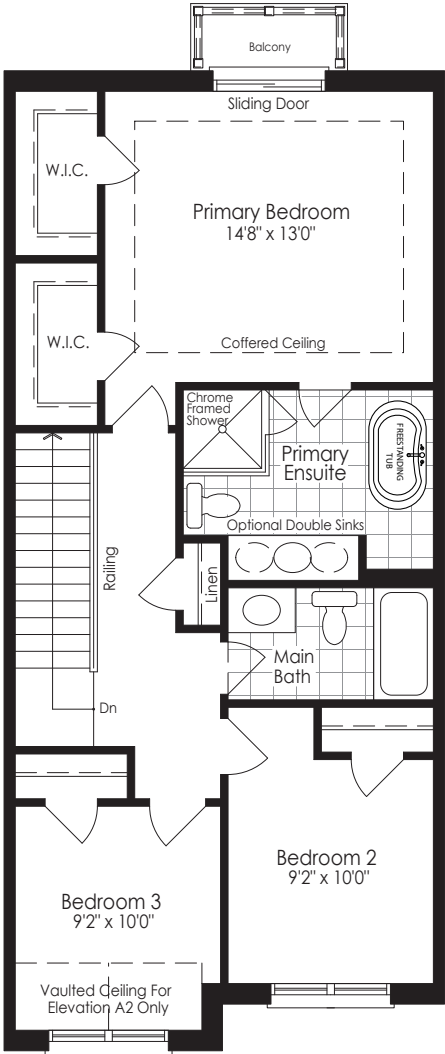
SECOND FLOOR Elevation A2
