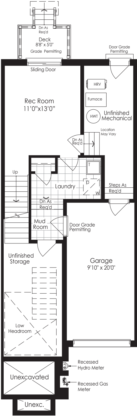
GROUND FLOOR Elevation B
