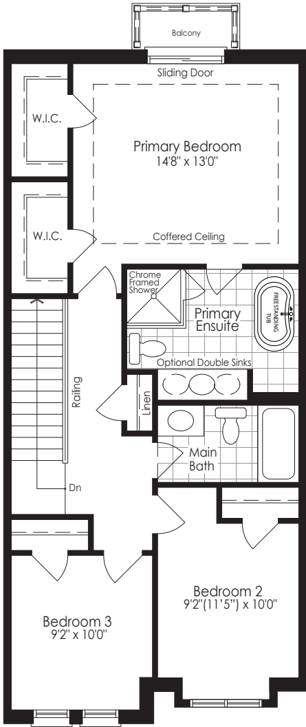
SECOND FLOOR Elevation B
