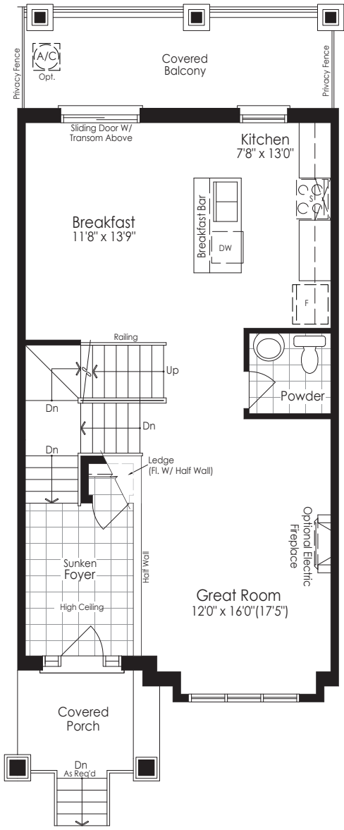
MAIN FLOOR Elevation B
