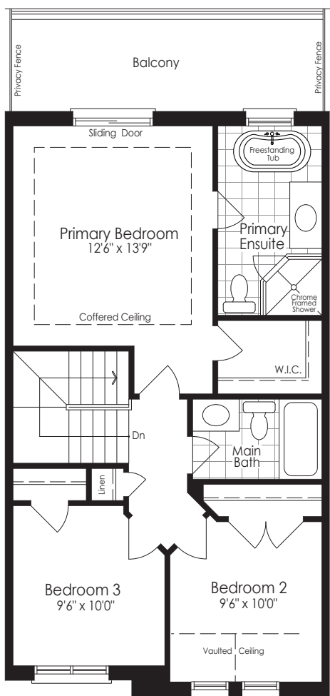
SECOND FLOOR Elevation B
