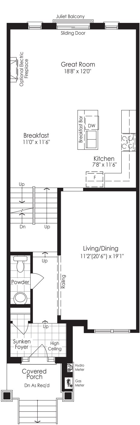
MAIN FLOOR Elevation A2
