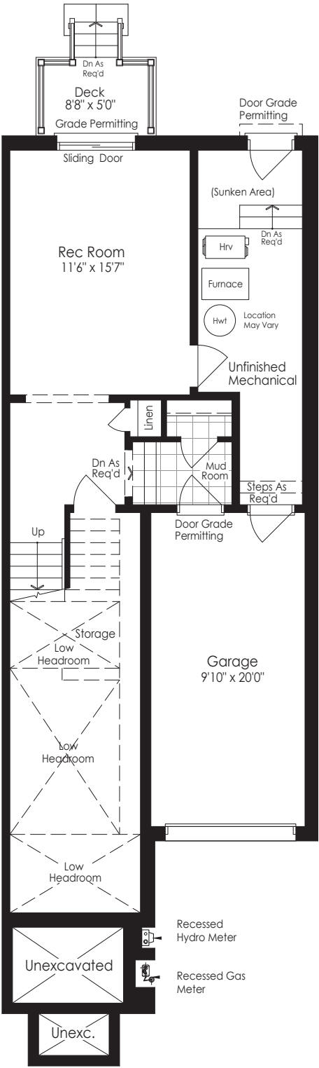
GROUND FLOOR Elevation A2
