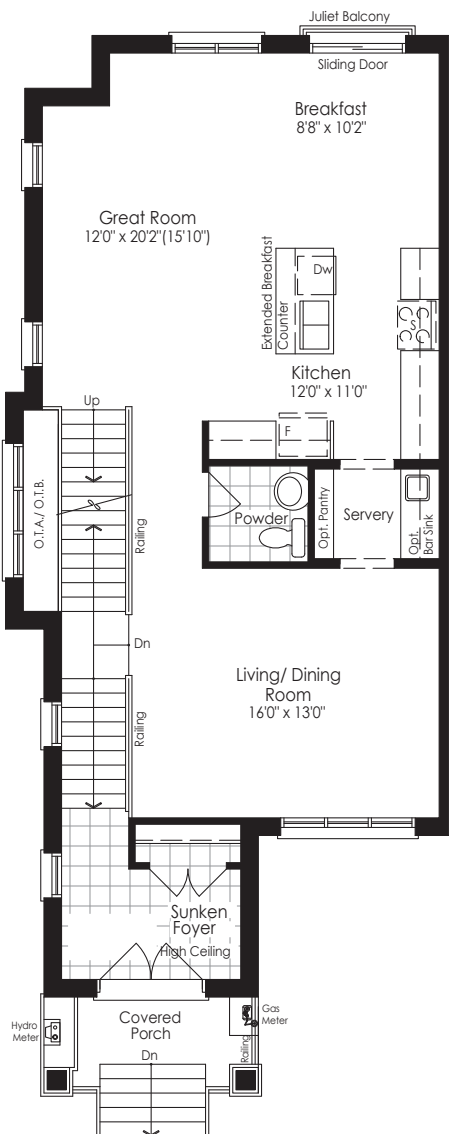
MAIN FLOOR Elevation B
