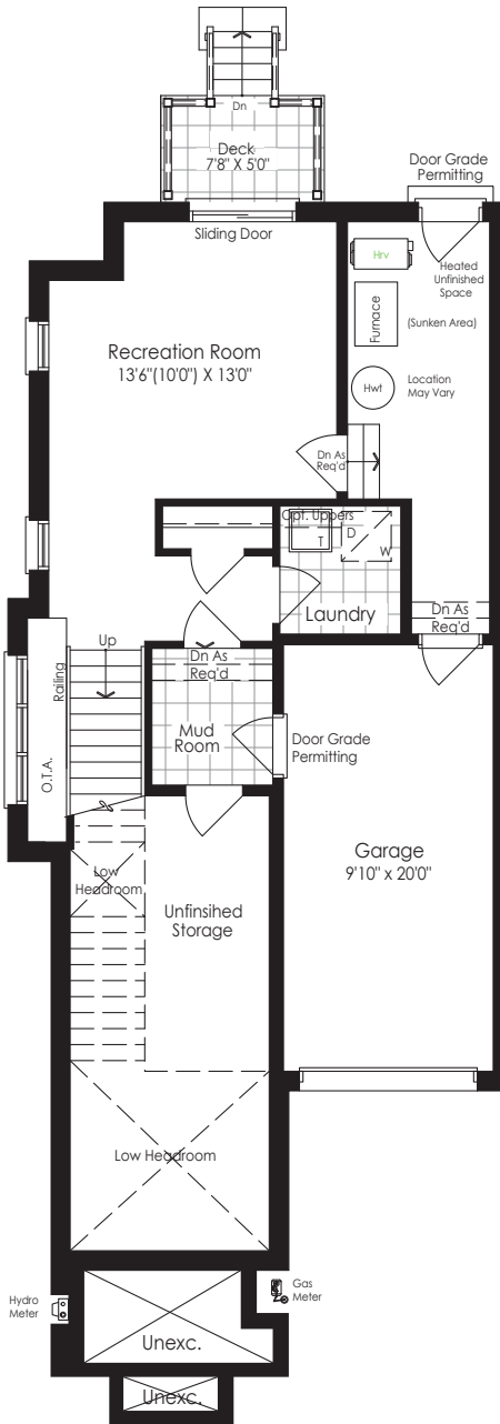
GROUND FLOOR Elevation B
