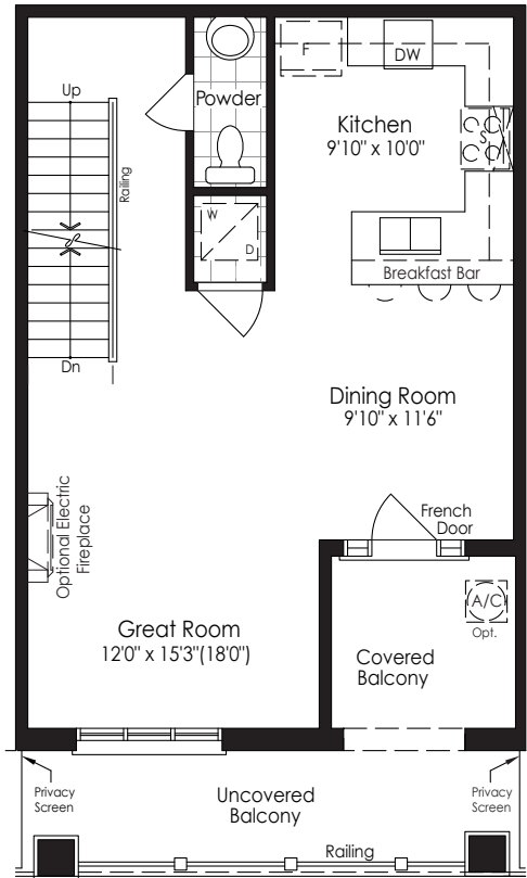
MAIN FLOOR Elevation A
