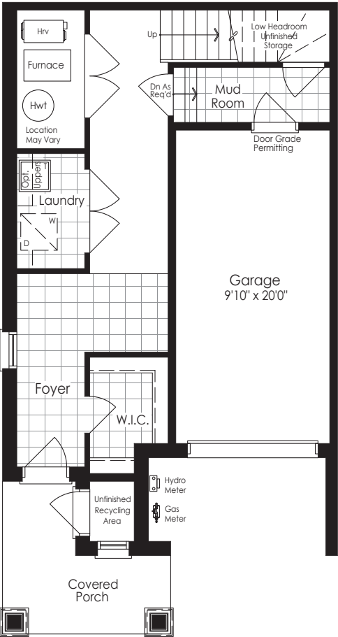
GROUND FLOOR Elevation A
