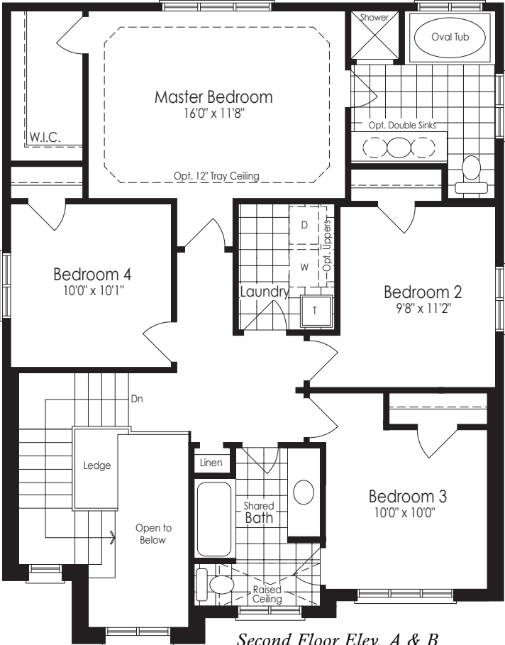
Second Floor Elev. A & B
