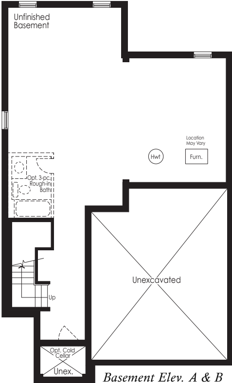
Basement Elev. A & B
