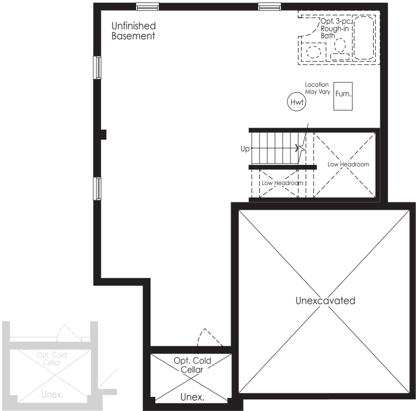
Basement Elev. A & B
