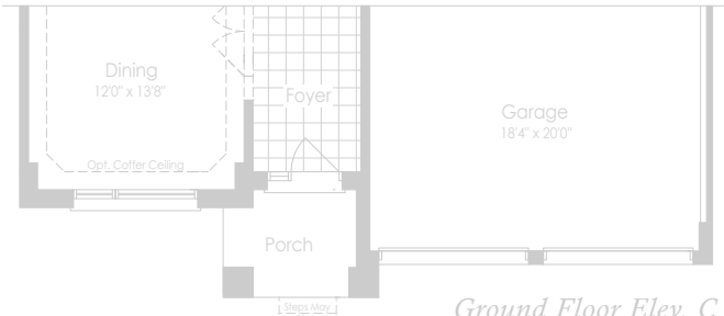
Ground Floor Elev. C
