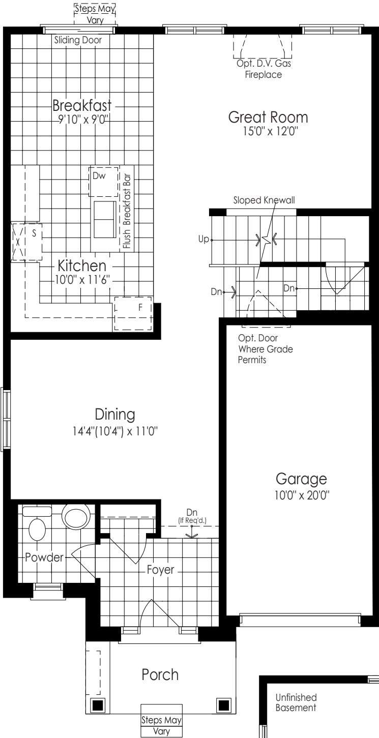
Ground Floor Elev. A & B
